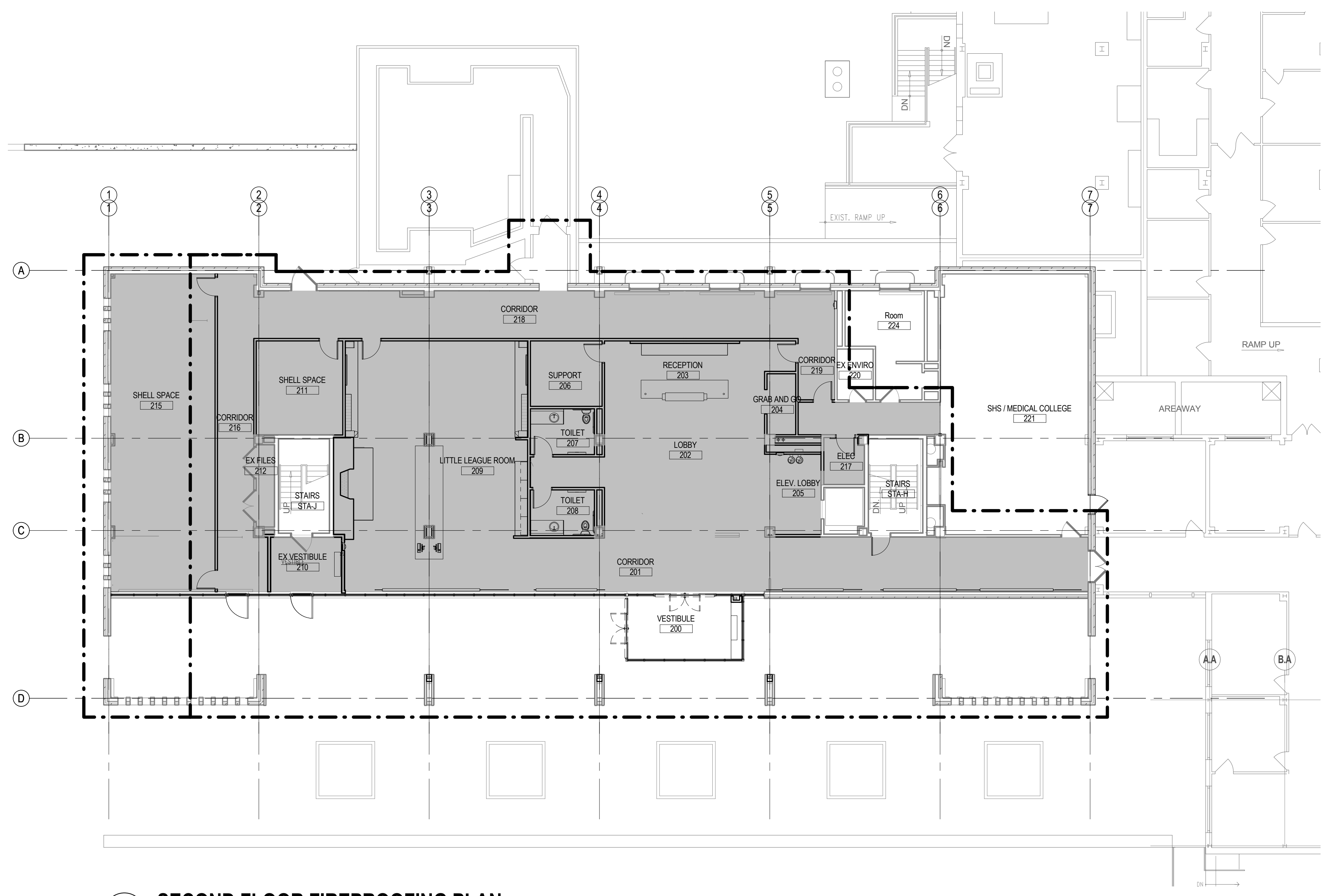
1 SECOND FLOOR FIREPROOFING PLAN GI-005 3/32" = 1'-0"
