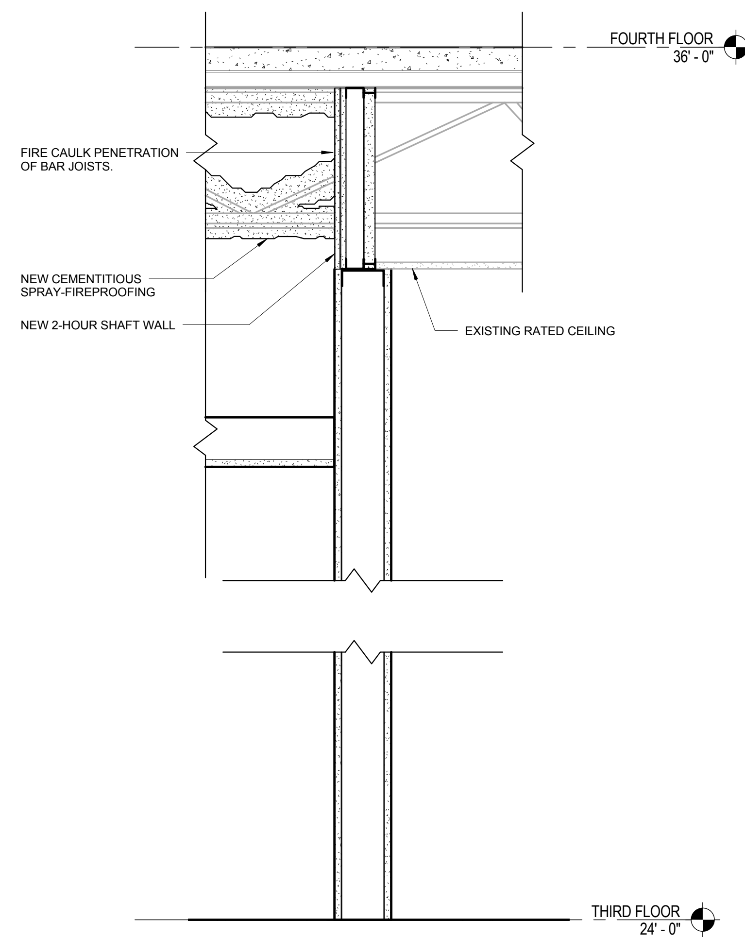
3 TRANSITION FROM NEW TO EXISTING FIRE RATING GI-005 1 1/2" = 1'-0"
