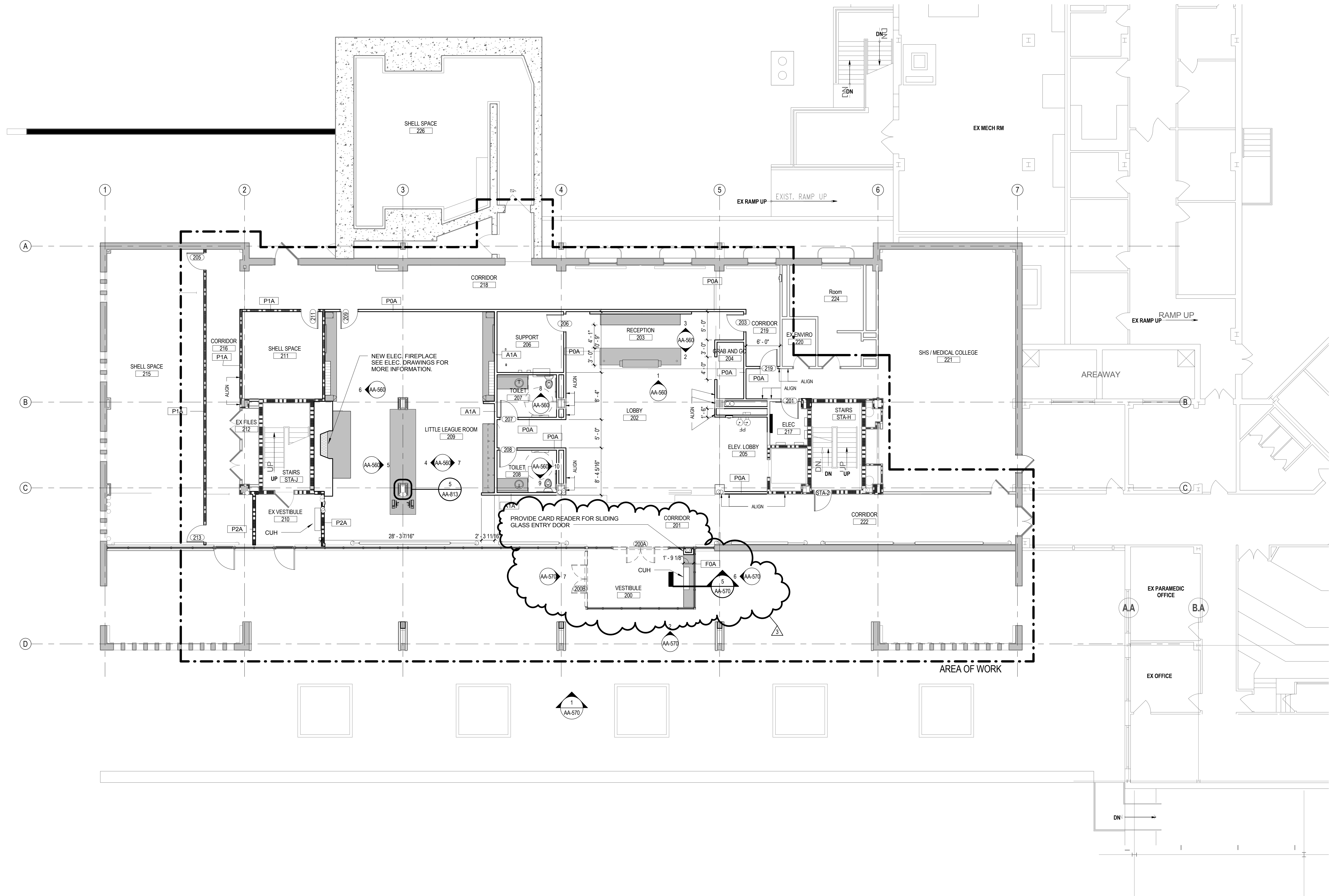
1 SECOND FLOOR ARCHITECTURAL PLAN 1/8" = 1'-0"
